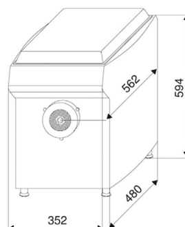
Dimensions Microlite
