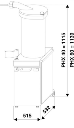
Dimensions PHX40 - PHX60
