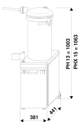
Dimensions PH13 - PHX15
