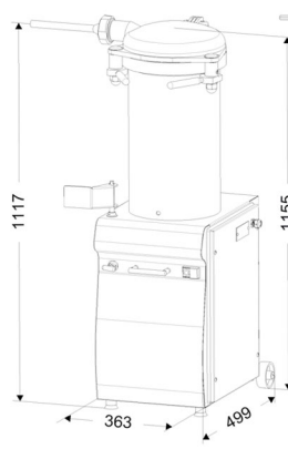
Dimensions PHX25
